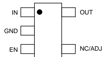
TSOT-23-5 (Top View)
